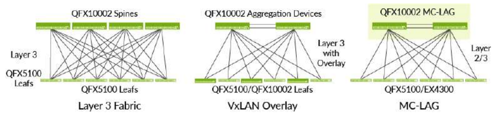
Figure 2: QFX10000 switches can be deployed in Layer 3 fabric, VxLAN overlay, or MC-LAG configurations.
